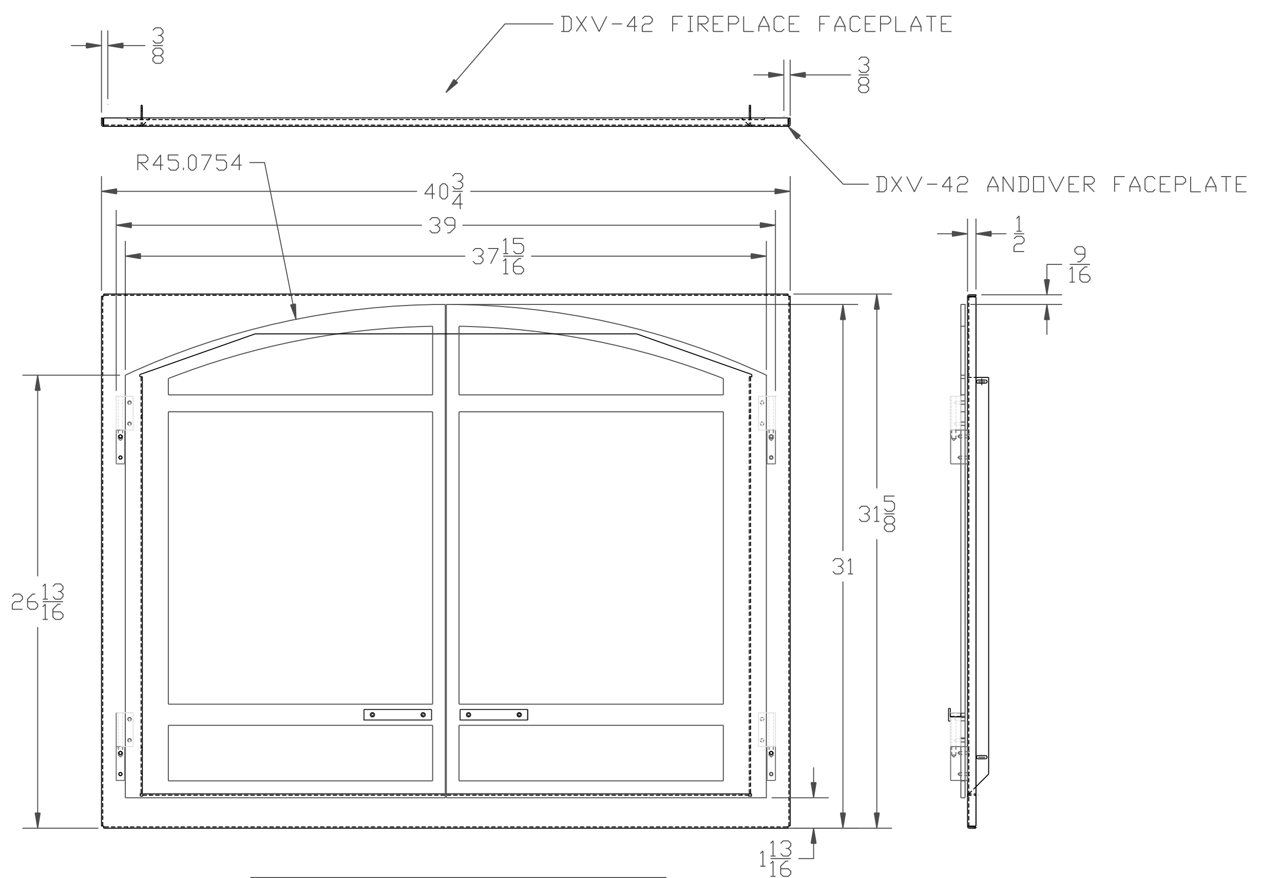
DXV-42 ANDOVER DIMENSIONS
